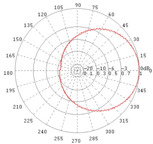
H-Ebene / H-Plane 80 MHz
