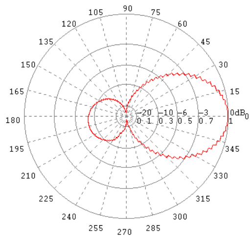
E-Ebene / E-Plane 80 MHz
