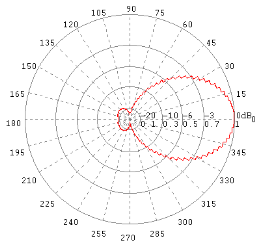
E-Ebene / E-Plane 100 MHz
