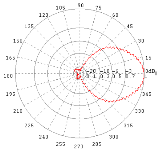
E-Ebene / E-Plane 300 MHz
