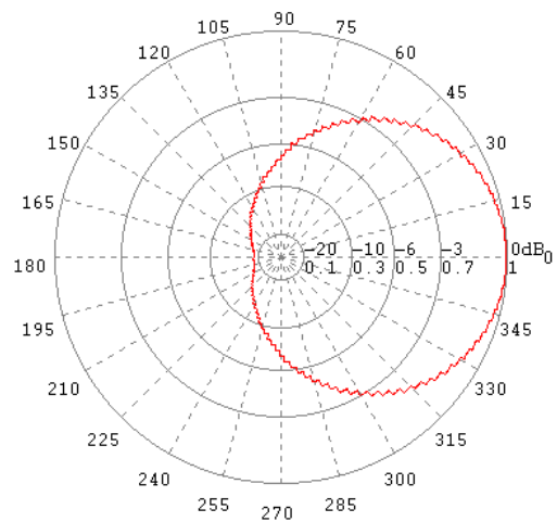
H-Ebene / H-Plane 100 MHz
