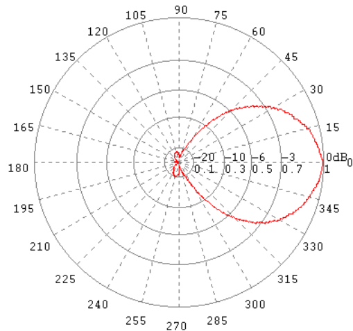
E-Ebene / E-Plane 800 MHz
