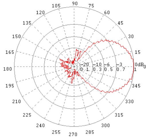
E-Ebene / E-Plane 600 MHz
