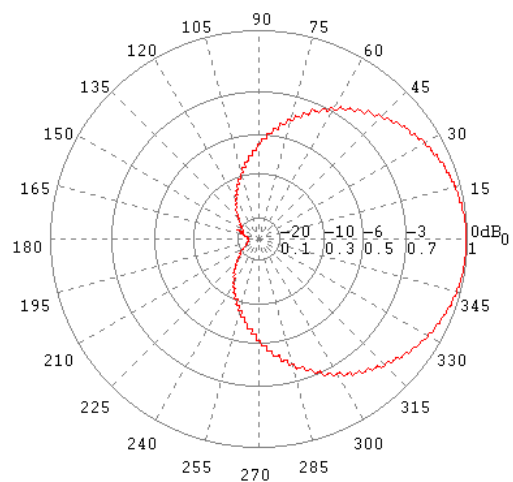
H-Ebene / H-Plane 120 MHz
