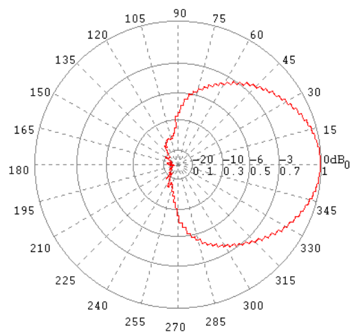
H-Ebene / H-Plane 400 MHz
