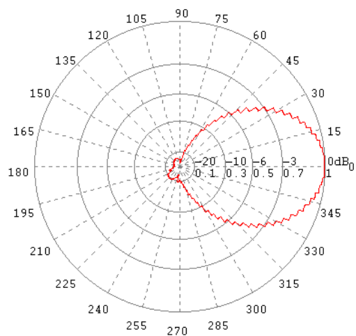
E-Ebene / E-Plane 120 MHz
